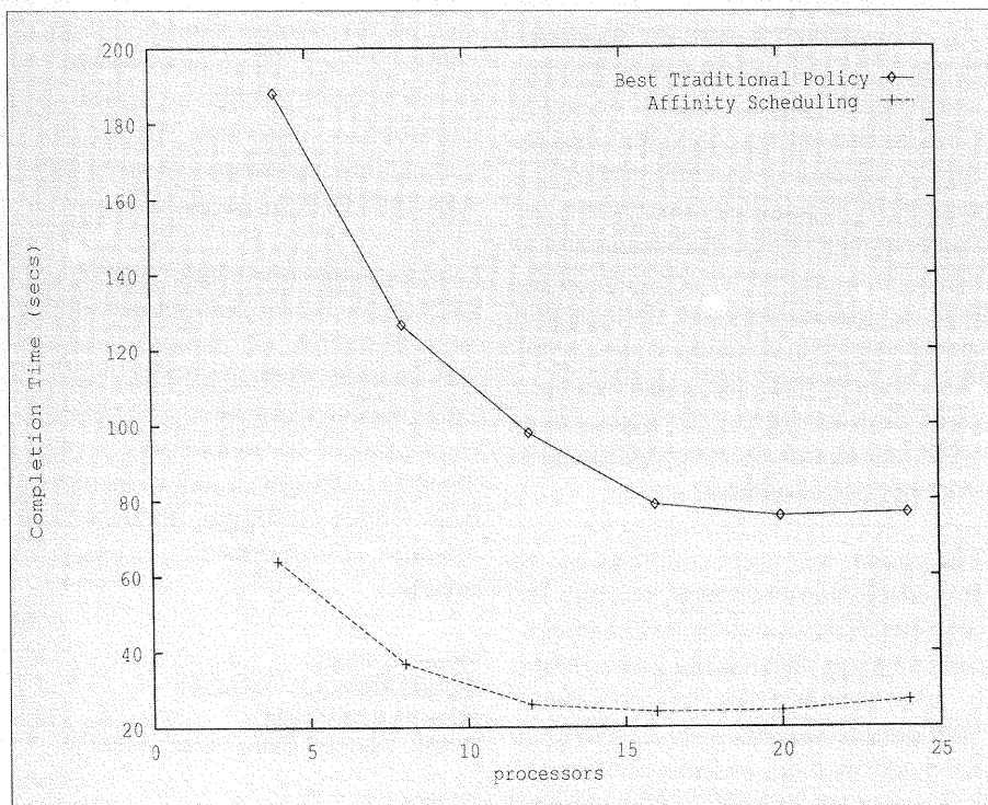
Gaussian elimination (1024 by 1024) on the KSR-1 multiprocessor.
